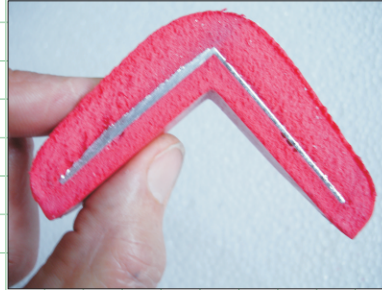
Aluminum Reinforced Strips Length: 39.4" Inside Dimensions: 2.0" x 2.0" Thickness: 3/4"
